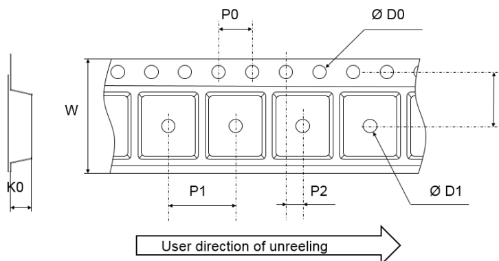
Figure 24. Tape outline
