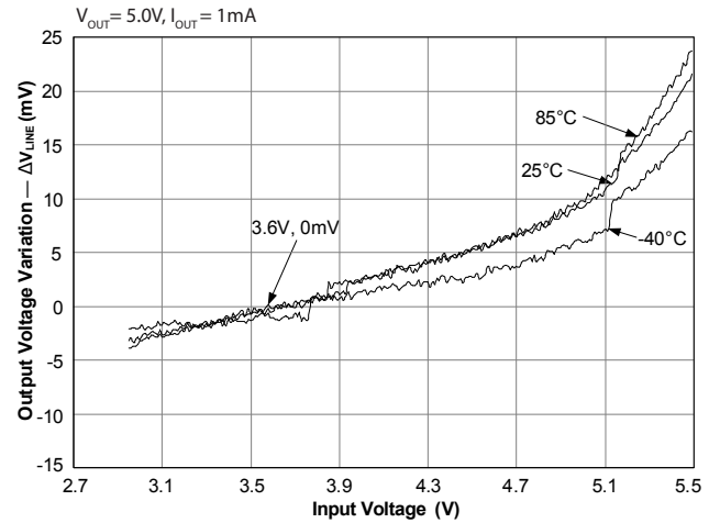
Line Regulation
