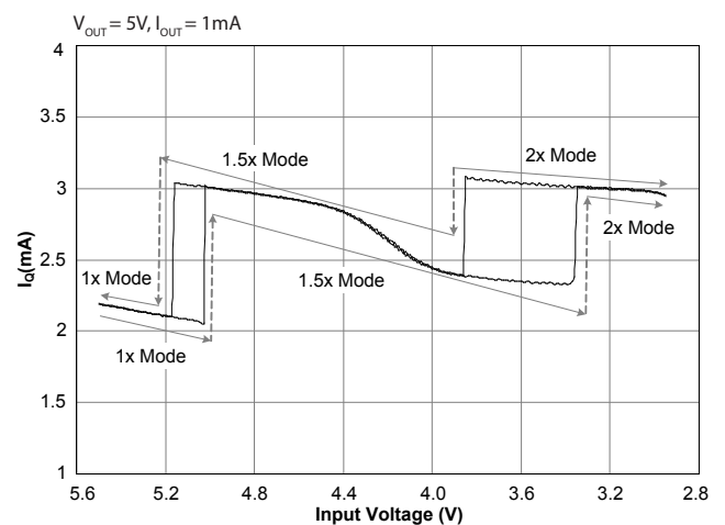
Quiescent Current
