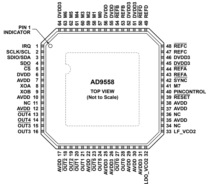
Figure 2. Pin Configuration
