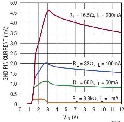
LT3062-3.3 GND Pin Current
