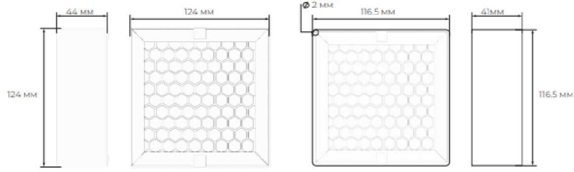
Filter size including the sealing foam.
