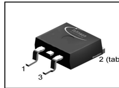
PG-TO263-3-2
