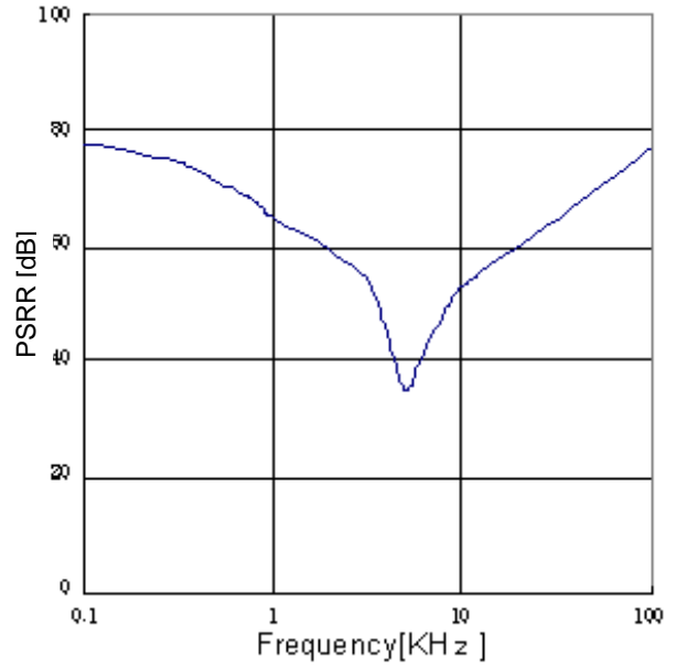
Figure 32. PSRR (Io=0mA)
