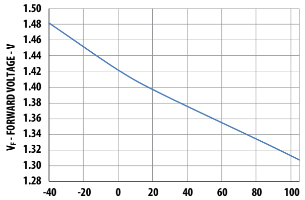
Figure 3: Typical V_F Versus Temperature
