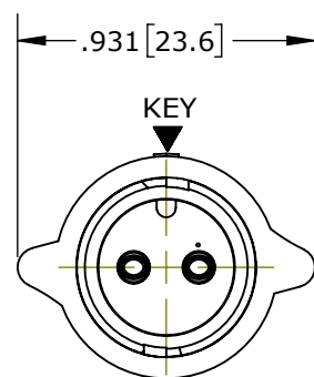
MATING FACE ASSY: W6380-2SG-P-3XX SHOWN
