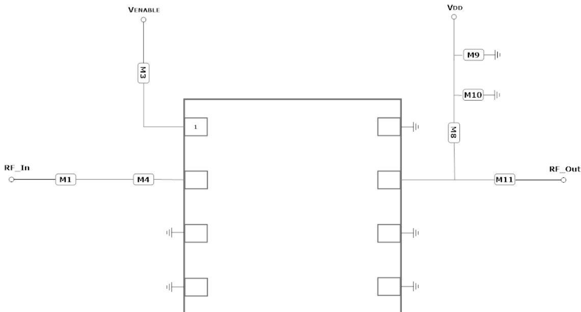
GRF2071-W Application Schematic
