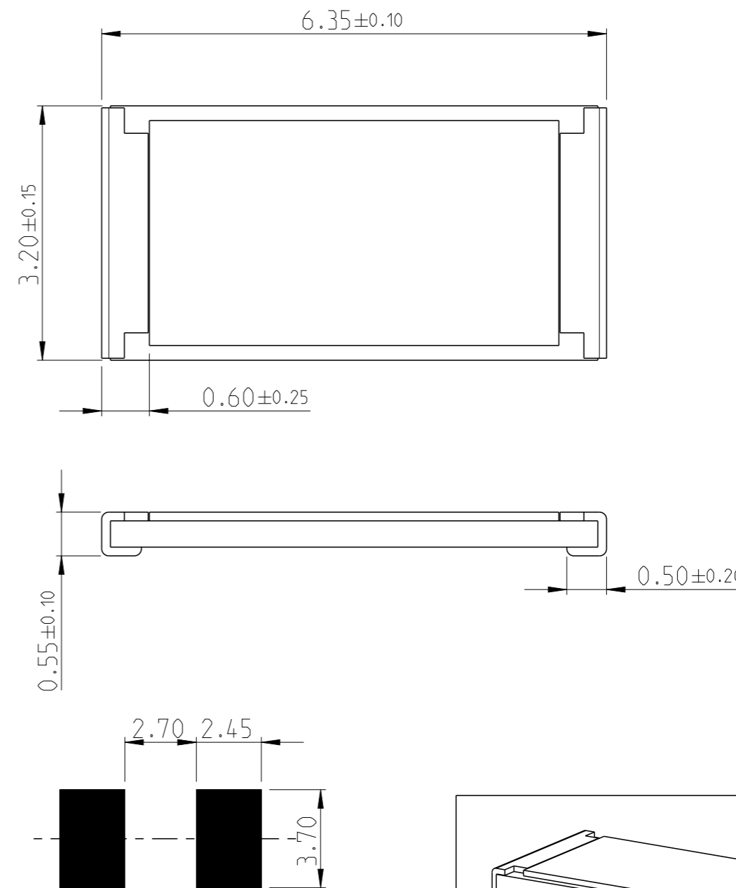
PDB LAYOUT PLAN
