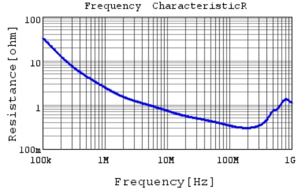
RDER72J102K2M1H03A R DCOV, 25degC
