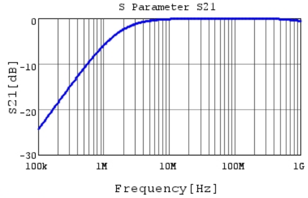
RDER72J102K2M1H03A S21 DCOV, 25degC
