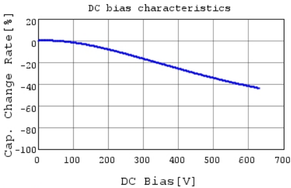
RDER72J102K2M1H03A C-DC bias capchange, 25.0
