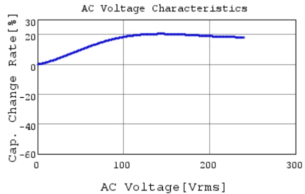
RDER72J102K2M1H03A C-AC Voltage capchange, I
