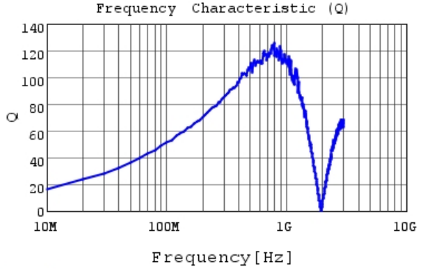
LQW2UAS47NJ00 Q
