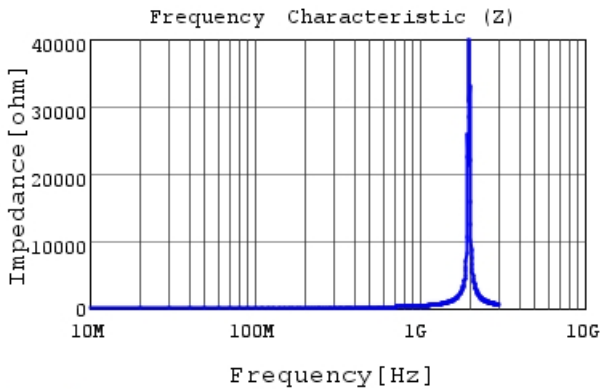
LQW2UAS47NJ00 |Z|
