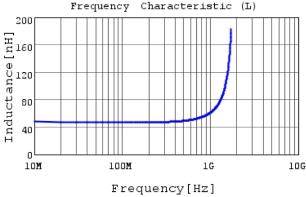
LQW2UAS47NJ00 L
