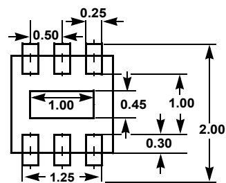
LAND PATTERN
