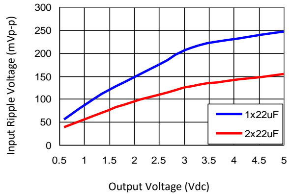
Figure 46. Input ripple voltage for various output voltages with 1x22 μF or 2x22 μF ceramic capacitors at the input (10A load). Input voltage is 12V.
