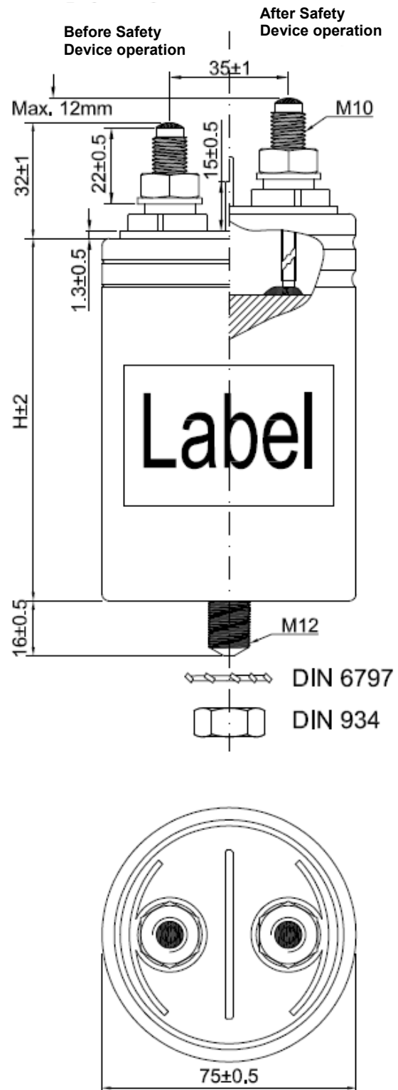
Figure 3: Series B32362
