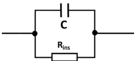
Figure 12: Insulation Resistance ( R_{ins} )
