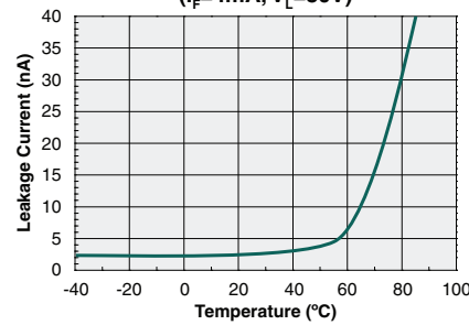
Leakage Current vs. Temperature Measured Across Pins 4 & 6 ( I_F=4mA, V_L=30V )
