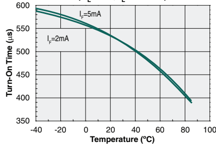
Typical Turn-On Time vs. Temperature ( V_L=10\text{V} , I_L=100\text{mA} )
