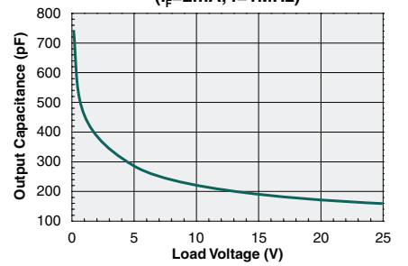
Output Capacitance vs. Load Voltage ( I_F=2mA, f=1MHz )
