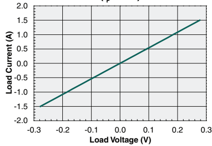
Typical Load Current vs. Load Voltage DC-Only Configuration ( I_F=0mA )
