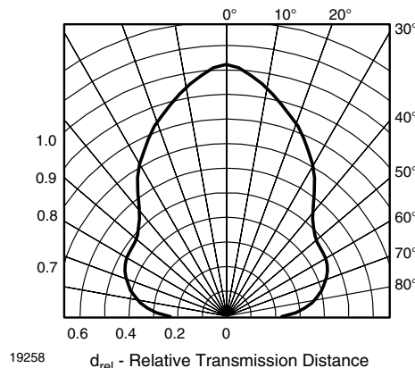
Fig. 12 - Horizontal Directivity
