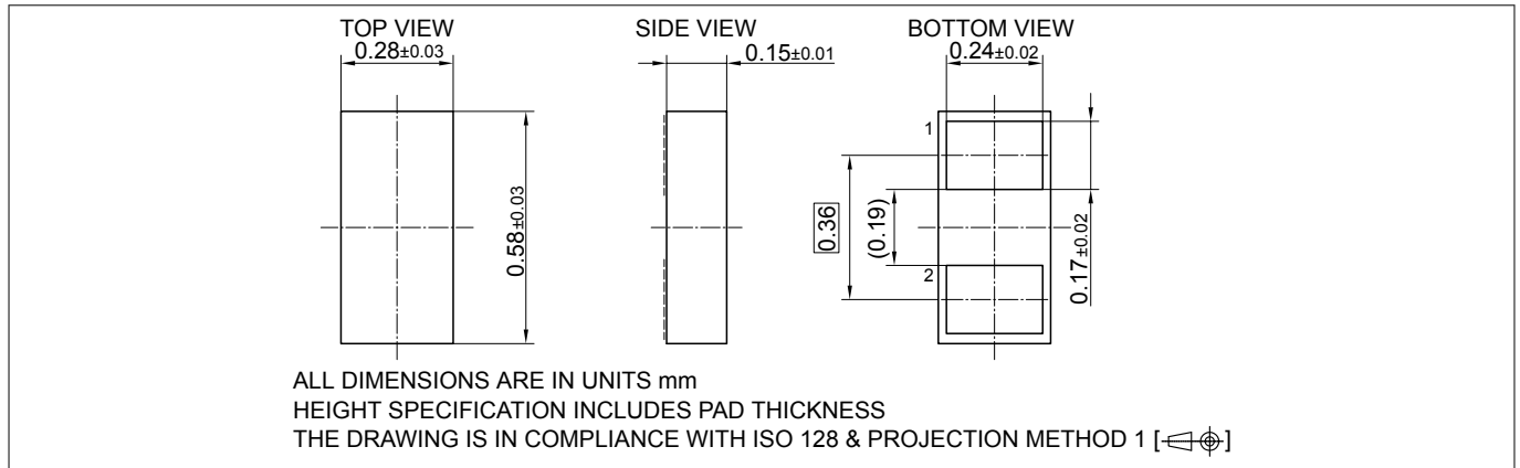
Figure 10 WLL-2-3 package
