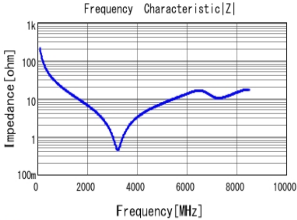
■ GRM1555C1H7R5DA01 |Z| DC0V, 25degC
