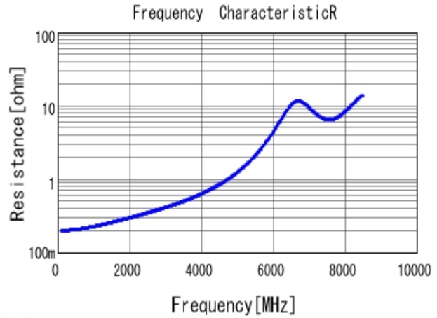
■ GRM1555C1H7R5DA01 R DC0V, 25degC
