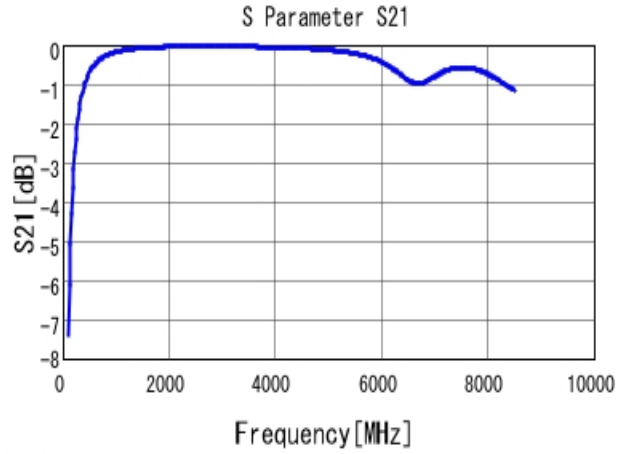
■ GRM1555C1H7R5DA01 S21 DCOV, 25degC
