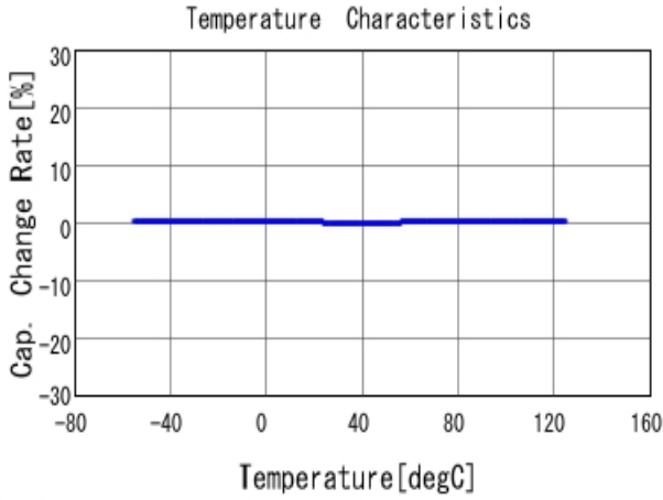
■ GRM1555C1H7R5DA01 C-Temp. capchange, DCOV, AC1Vrms
