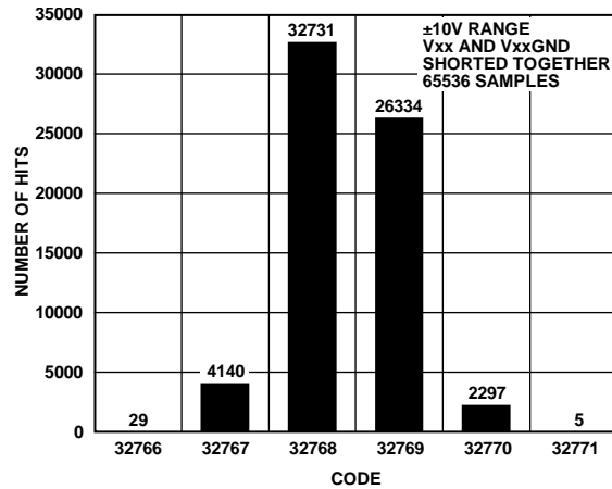
Figure 17. DC Histogram of Codes at Code Center, \pm 10 V Range
