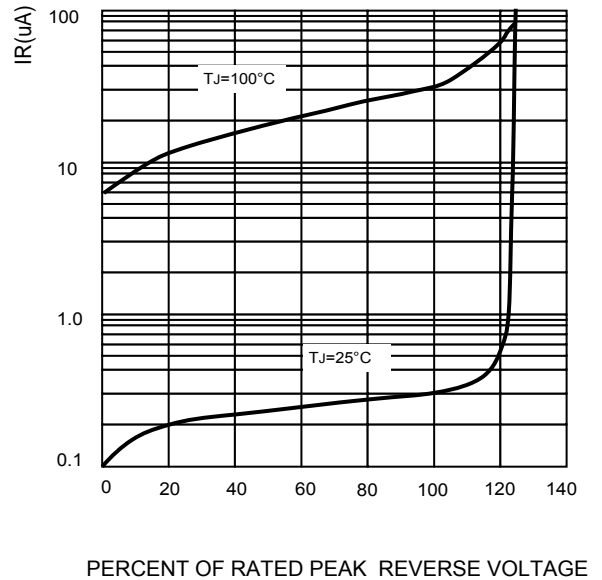
FIG.4-TYPICAL REVERSE CHARACTERISTICS
