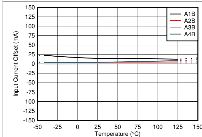
Figure 7-3. TMCS1101AxB Input Offset Current vs Temperature
