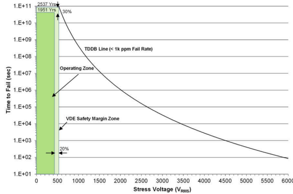
Figure 9-1. Insulation Lifetime
