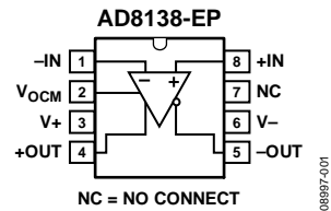
Figure 6. Pin Configuration
