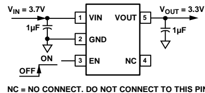
Figure 1. TSOT ADP151-EP with Fixed Output Voltage, 3.3 V
