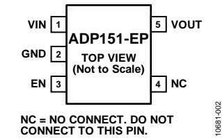
Figure 2. 5-Lead TSOT Pin Configuration
