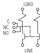
BREAKER SHOWN IN OFF POSITION
