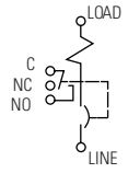
BREAKER SHOWN IN OFF POSITION
