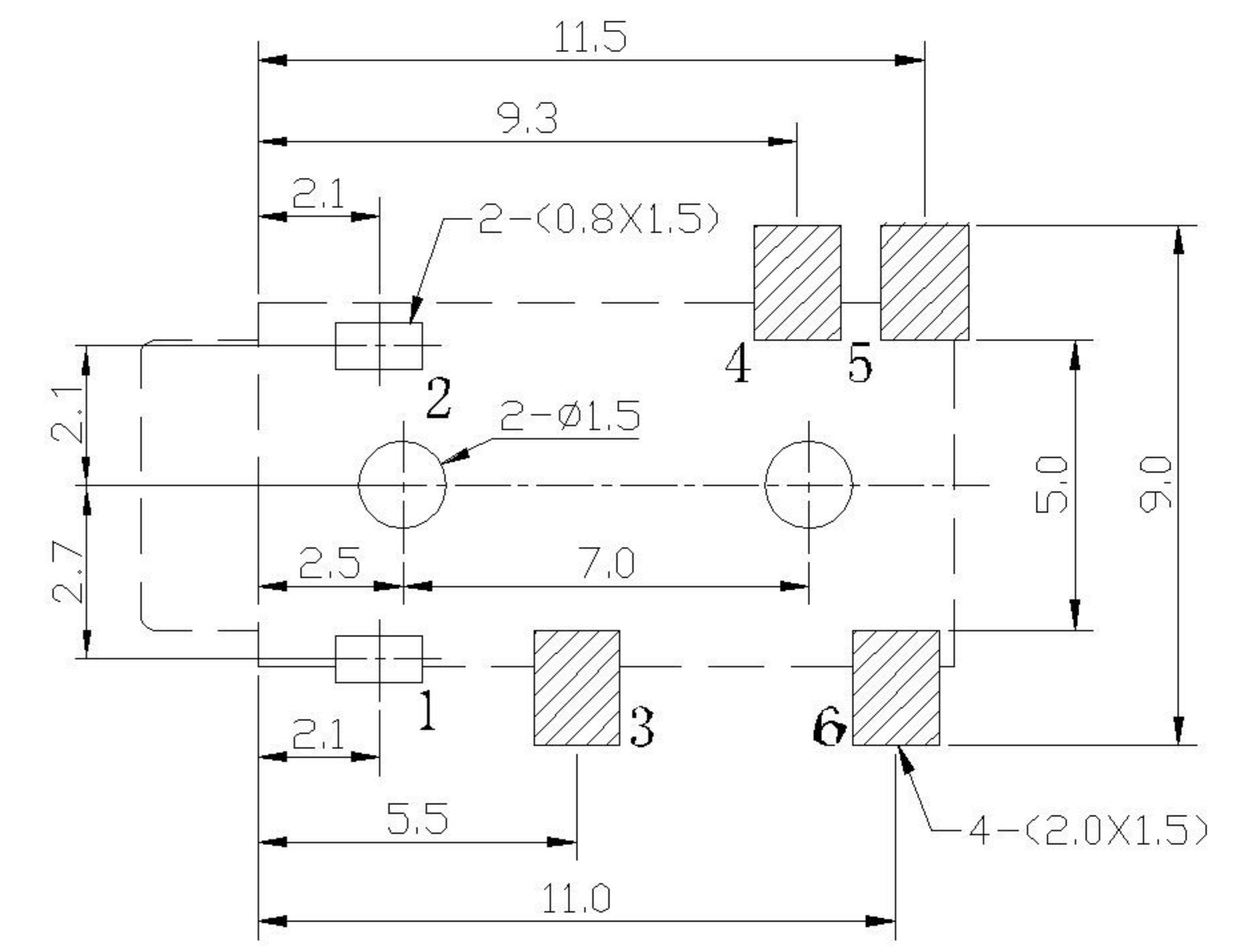
P.C.B LAYOUT TOP VIEW
