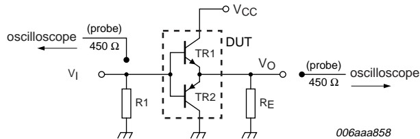
Fig 17. Test circuit for switching times
