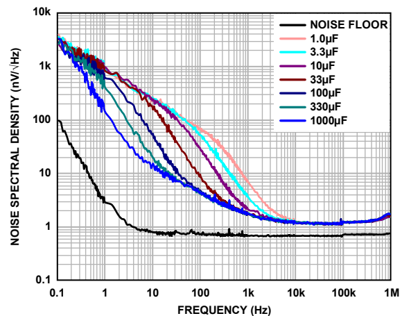
Figure 2. Noise Spectral Density for Different Values of C_{\text{BY}}
