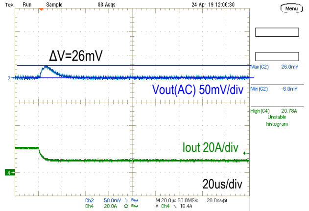
Step Load Transient Response (Vin=5.0V, Vout=0.7V, Cload=660uF, Iout=20 to 10A 1.0A/us) Trace 2=Vout(AC) 50mV/div, Trace 4=Iout 20A/div, 20us/div
