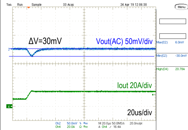
Step Load Transient Response (Vin=5.0V, Vout=0.7V, Cload=660uF, Iout=10A to 20A 1.0A/us) Trace 2=Vout(AC) 50mV/div, Trace 4=Iout 20A/div, 20us/div
