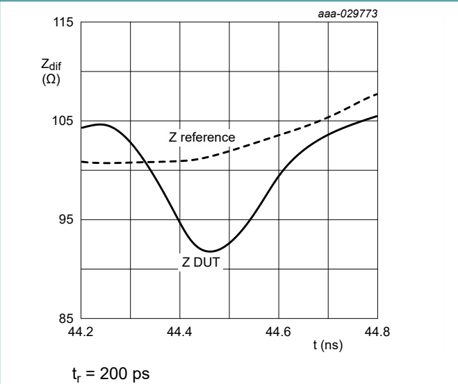
t_r = 200 ps Fig. 4. Differential Time Domain Reflectometer (TDR) plot; typical values
