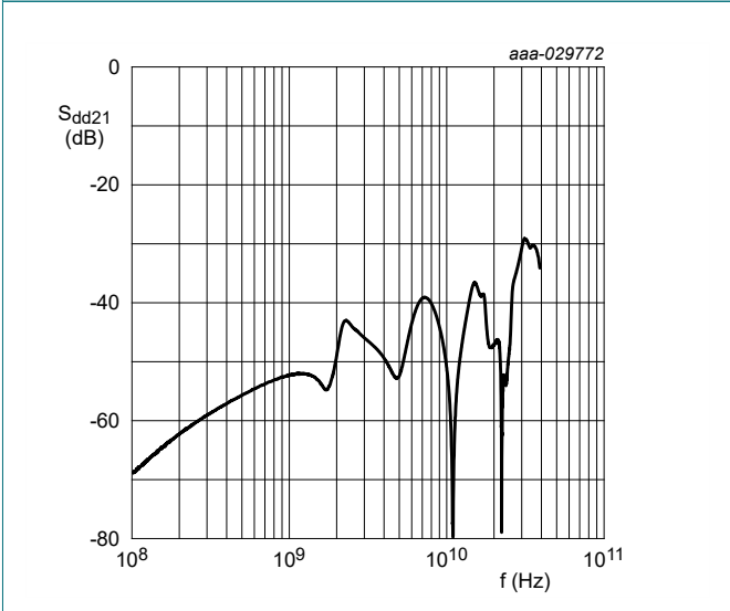
CH1 to CH2 Fig. 3. Differential crosstalk; typical values
