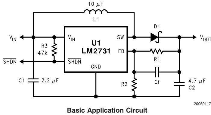
Basic Application Circuit
