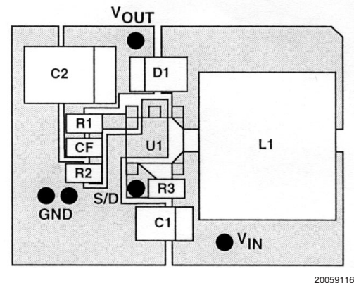
Recommended PCB Component Layout
