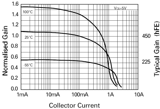
Collector Current h_{FE} vs I_C
