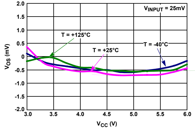
FIGURE 42. AUXILIARY V_{BUS} V_{OS} vs V_{CC}
