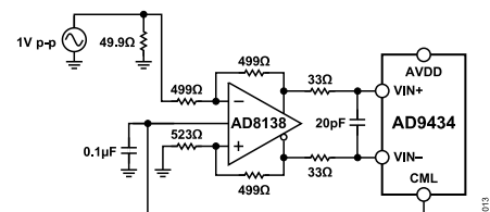
Figure 41. Differential Input Configuration Using the AD8138
