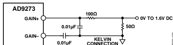
Figure 52. Single-Ended GAIN \pm Pins Configuration
