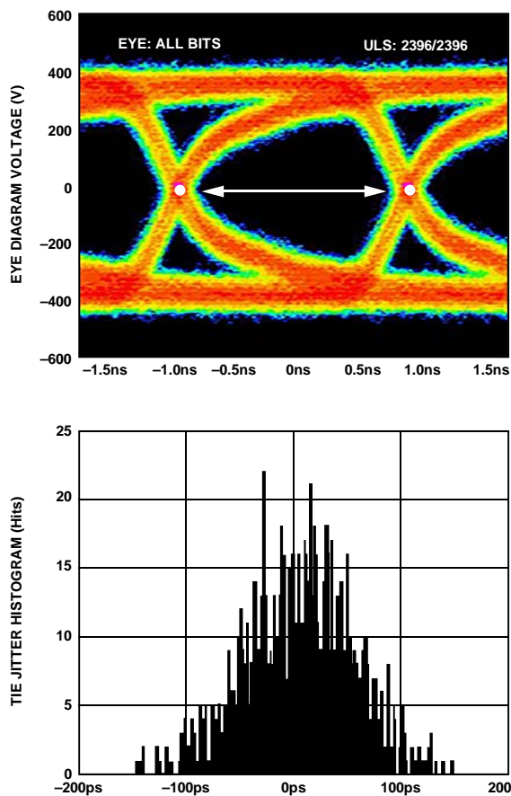
Figure 67. Data Eye for LVDS Outputs in ANSI-644 Mode with 100 \Omega Termination Resistor and Trace Lengths of Greater than 24 Inches on Standard FR-4
