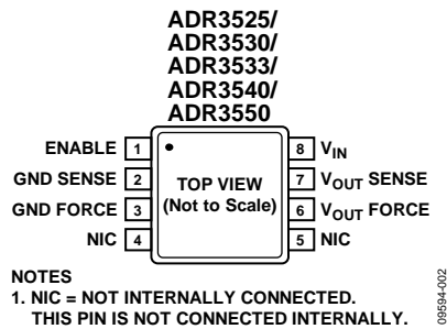
Figure 2. Pin Configuration
