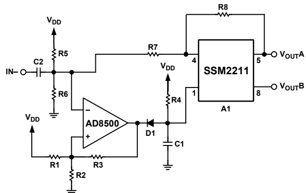
Figure 47. Automatic Shutdown Circuit
