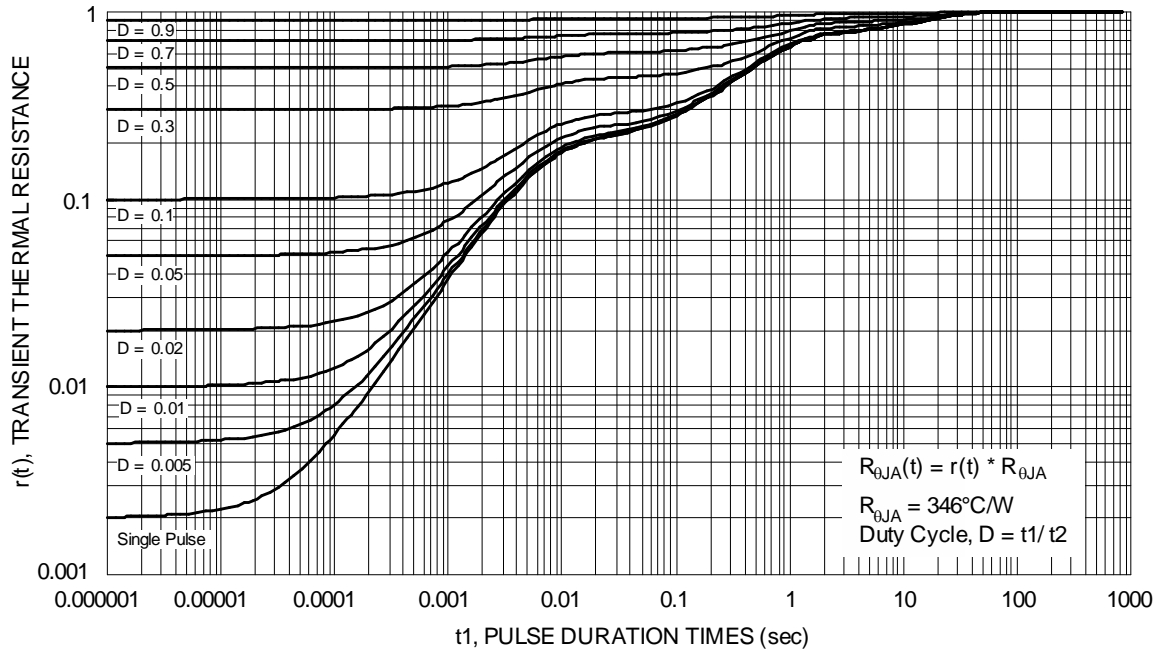
Figure 15 Transient Thermal Resistance
