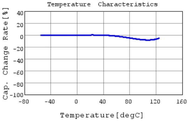
GRM21BR72A103KA01 C-Temp. capchange, DC0.0V,
