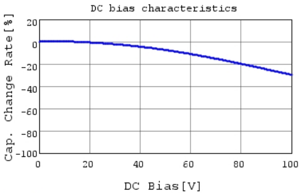
GRM21BR72A103KA01 C-DC bias capchange, 25.0c
