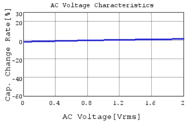
GRM21BR72A103KA01 C-AC Voltage capchange, Dc
