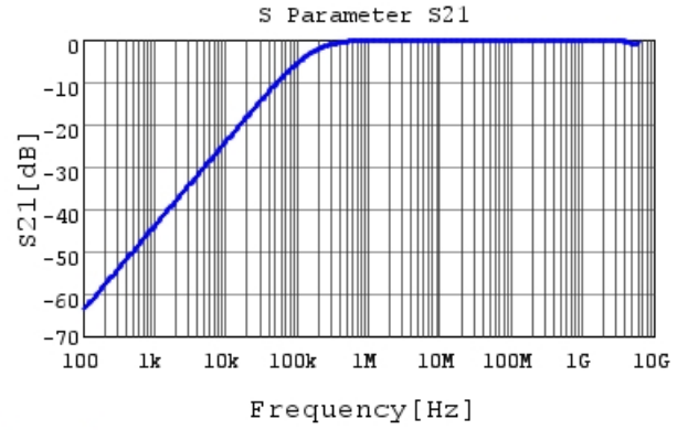
GRM21BR72A103KA01 S21 DC0V, 25degC
