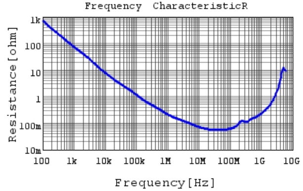
GRM21BR72A103KA01 R DCOV, 25degC
