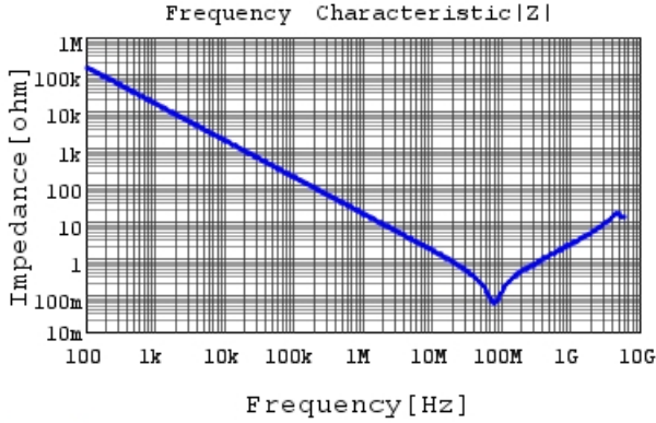
GRM21BR72A103KA01 |Z| DCOV, 25degC
