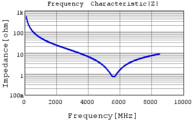
GRM0335C1H3R0CA01 |Z| DCOV, 25degC
