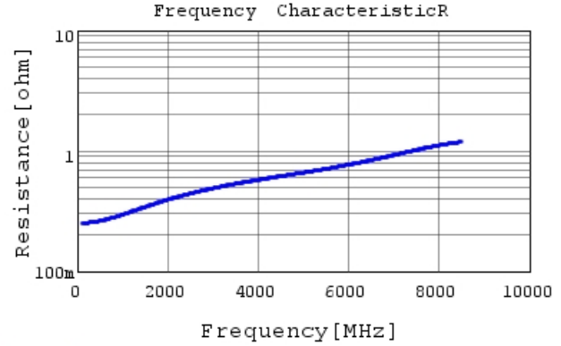
GRM0335C1H3R0CA01 R DCOV, 25degC
