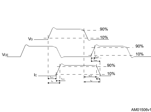
Figure 35. Switching waveform
