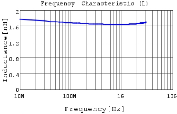
LQG18HN1N8S00 L
