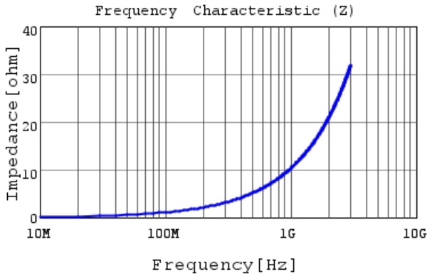
LQG18HN1N8S00 |Z|
