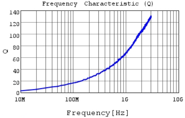
LQG18HN1N8S00 Q
