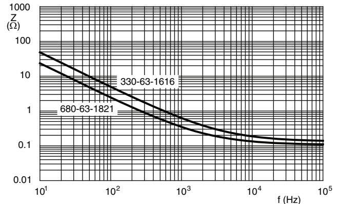
Fig. 12 - Typical impedance Z as a function of frequency at 20 °C
