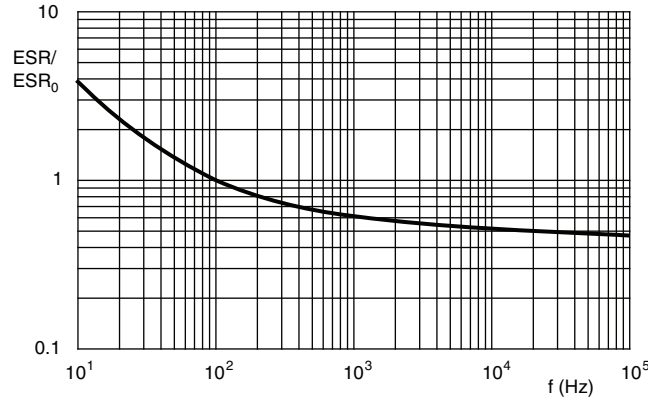
Fig. 8 - Typical multiplier ESR as a function of frequency at 20 °C
