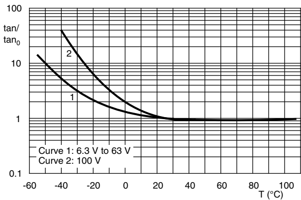
Fig. 9 - Typical multiplier of dissipation factor \tan \delta as a function of temperature at 20 °C at 100 Hz
