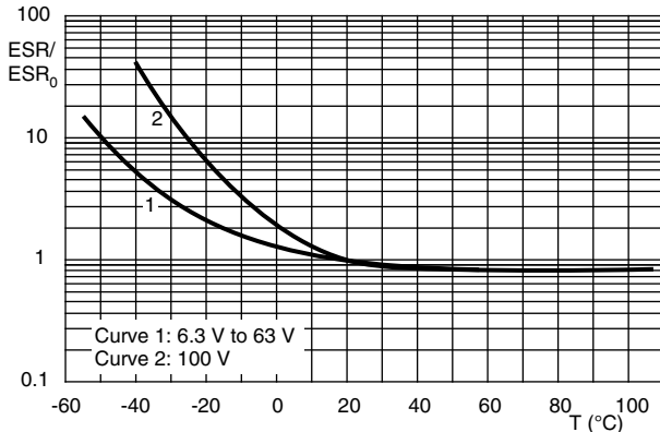
Fig. 7 - Typical multiplier of ESR as a function of temperature at 100 Hz
