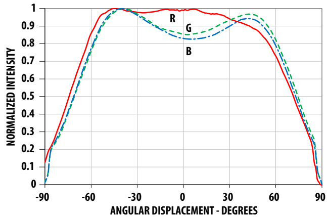
Figure 6 Radiation Pattern
