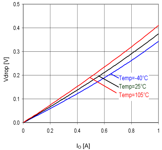
Figure 34. Minimum dropout Voltage 2 (V CC =2.4V, T a =25°C)
