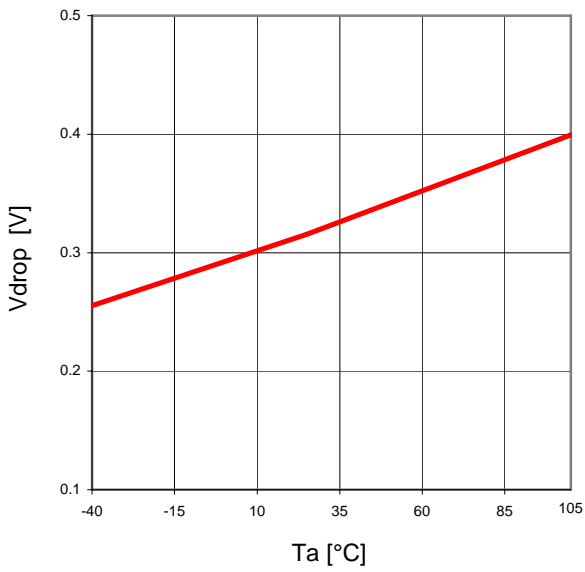
Figure 33. T a -V drop (V CC =6V, I o =0.3A)
