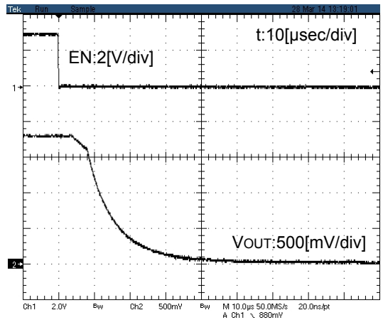
Figure.53 Turn off response 9 (BUS1DJC3GWZ VIN=1.8V)
