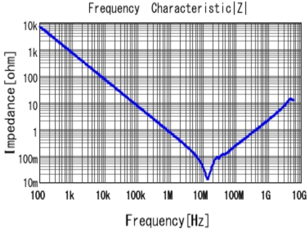
GCM21BR71H224KA37 |Z| DCOV, 25degC
