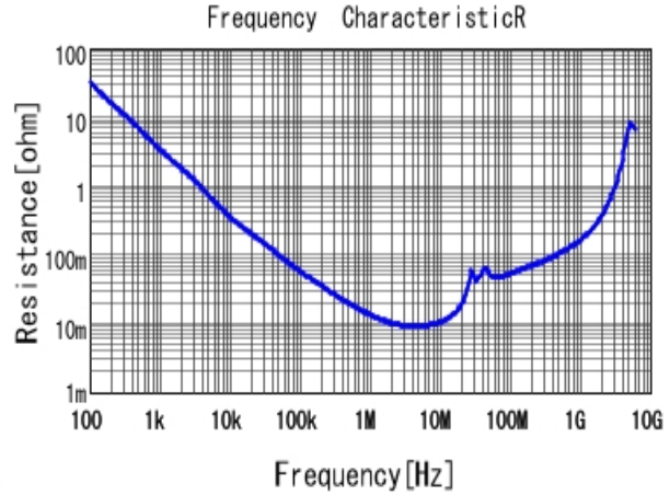
GCM21BR71H224KA37 R DCOV, 25degC
