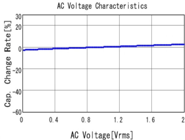
GCM21BR71H224KA37 C-AC Voltage capchange, DCOV, 25.0d
