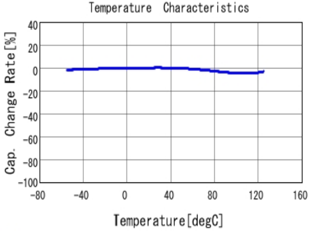
■ GCM21BR71H224KA37 C-Temp. capchange, DC0.0V, AC1.0V r m
