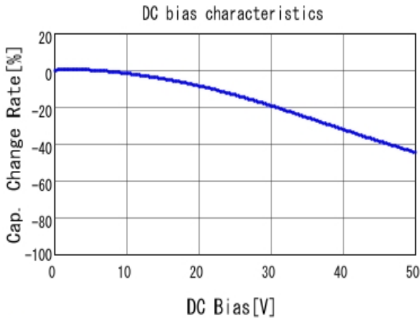
GCM21BR71H224KA37 C-DC bias capchange, 25.0degC, AC1.
