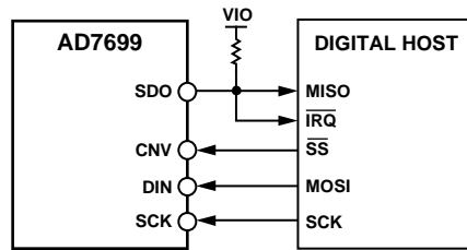
Figure 41. Connection Diagram for the AD7699 with a Busy Indicator
